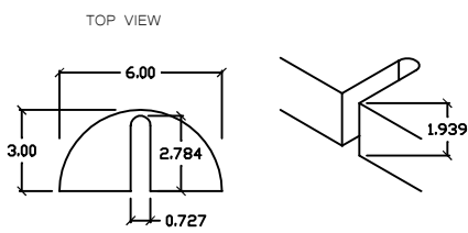
MOUNTING SLOT DETAIL SCALE 2:1 ALL DIMS NOMINAL
