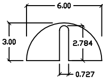
MOUNTING SLOT DETAIL SCALE 2:1
