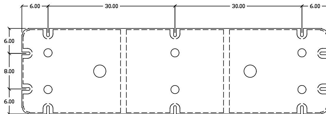
MOUNTING SLOT DETAIL SCALE 2:1
