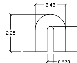
MOUNTING SLOT DETAIL SCALE 2:1
