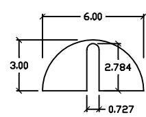
MOUNTING SLOT DETAIL SCALE 2:1
