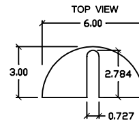
MOUNTING SLOT DETAIL SCALE 2:1 ALL DIMS NOMINAL
