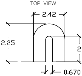
MOUNTING SLOT DETAIL SCALE 2:1
