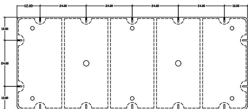
MOUNTING SLOT DETAIL SCALE 2:1 ALL DIMS NOMINAL
