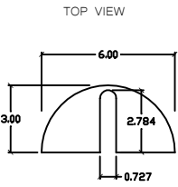
MOUNTING SLOT DETAIL SCALE 2:1 ALL DIMS NOMINAL
