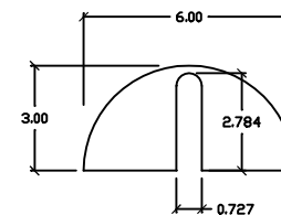
MOUNTING SLOT DETAIL SCALE 2:1 ALL DIMS NOMINAL
